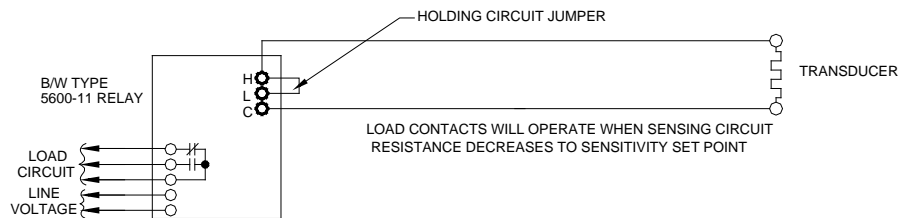
DIAGRAM D CONTROL FROM RESISTIVE TRANSDUCER 5600-11 DIRECT OPERATION LOAD ACTUATION ON DECREASING RESISTANCE
